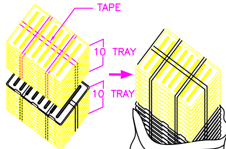
TOTAL 20 TRAY
