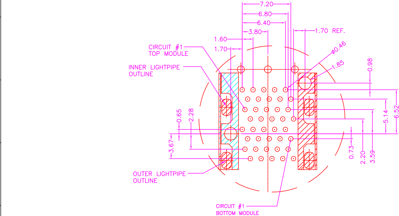
P.C.B. LAYOUT TOP VIEW ±0.05
