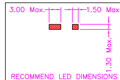
LED CLEARANCE REQUIREMENTS
