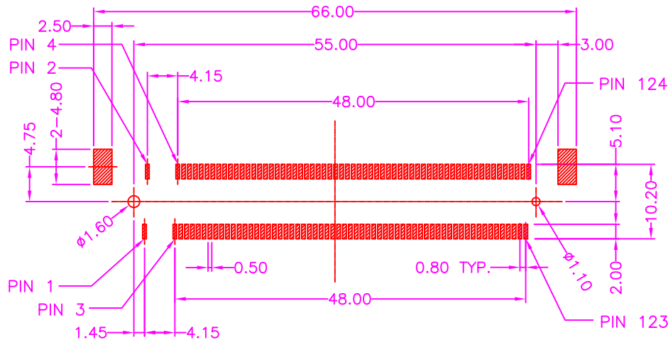
P.C.B LAYOUT TOP VIEW ±0.05
