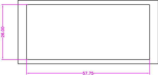
BEZEL CUT-OUT CENTER SPACING DETAIL BEZEL THICKNESS:0.8-2.6
