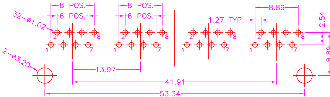
P.C.B. LAYOUT TOP VIEW ±0.05
