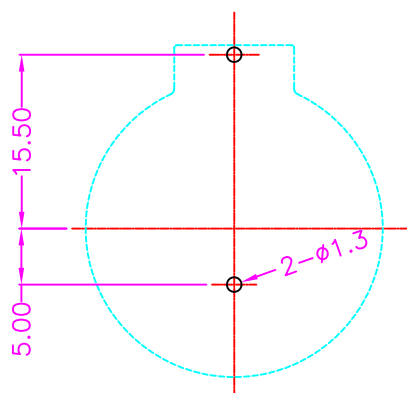
P.C.B. LAYOUT TOP VIEW ±0.05
