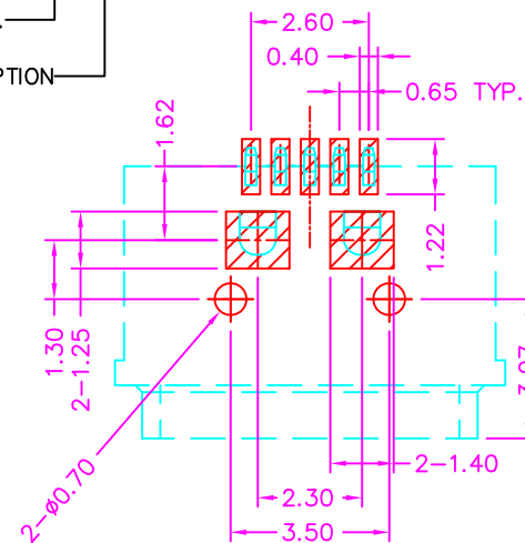
P.C.B. LAYOUT TOP VIEW ±0.05
