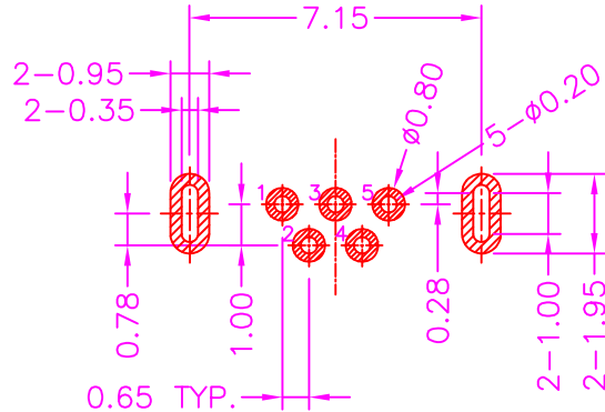
P.C.B LAYOUT TOP VIEW ±0.05
