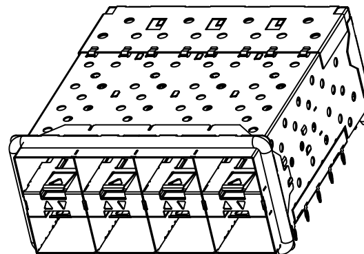
024BP-0*C-132 WITH INNER LIGHT PIPES
