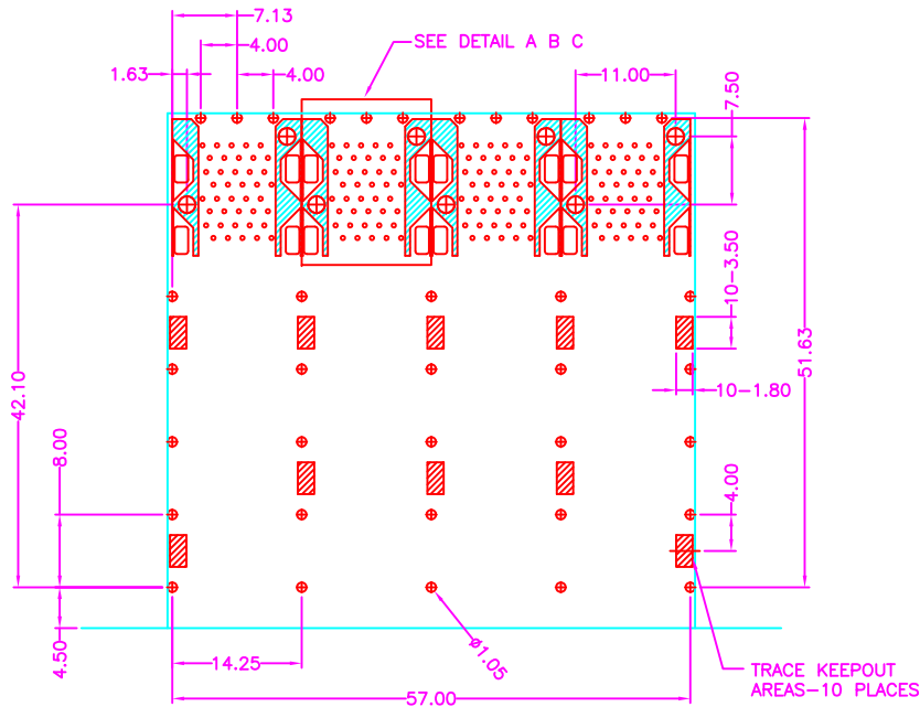
P.C.B LAYOUT TOP VIEW ±0.05
