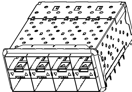
024BP-0*C-122 WITH OUTER LIGHT PIPES
